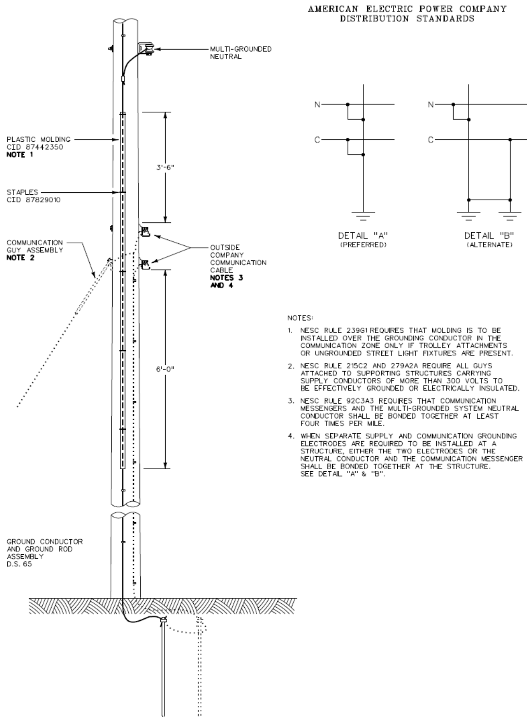
GROUND WIRE INSTALLATION JOINT USE POLES
